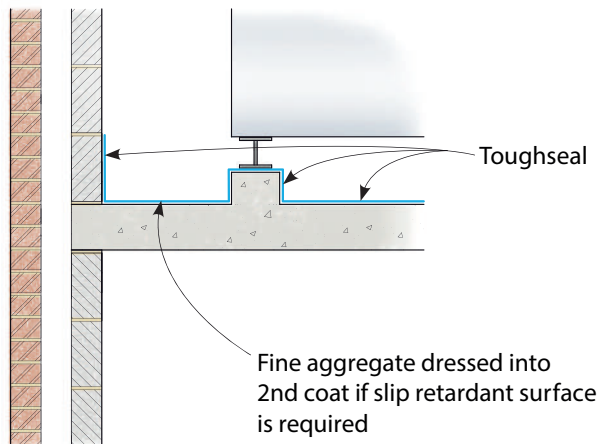
Detail 1 - Plant room detail, horizontal wearing surface
