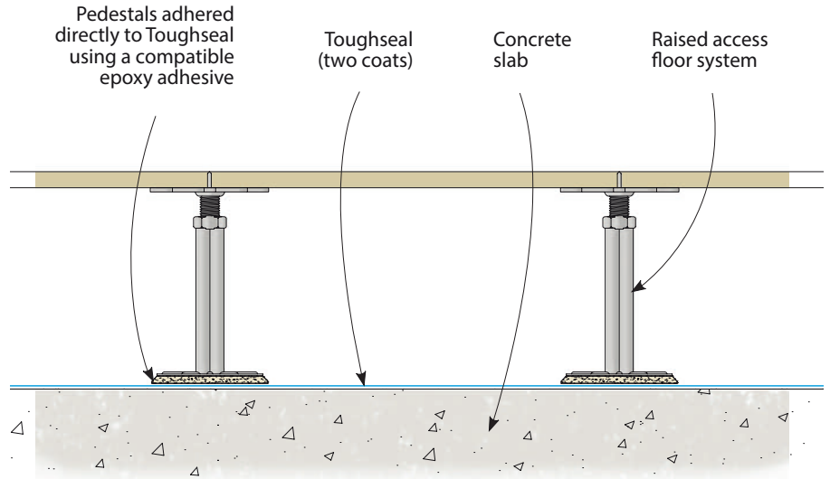
Raised access floor
